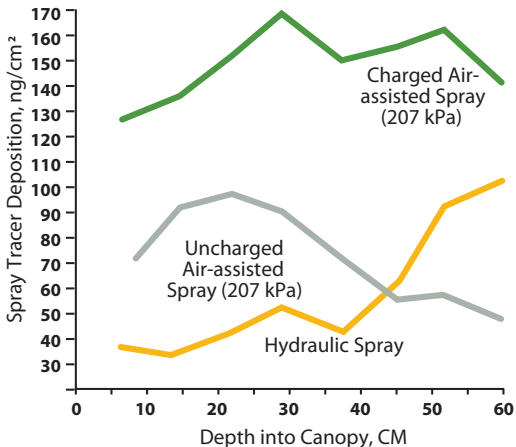
Spray Deposition vs. Depth into Canopy on Cotton Broadcast Spray, Fluorometric Analysis
